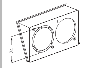
Insert for two XLR round plugs, D series, Speakon series NL 4 MP (Neutrik) 0055 00
