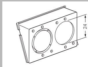
Insert for two XLR round plugs C series 0092 00
